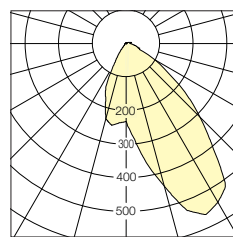
1 x 54 W lamp diffuser PMMA, transopal, impact strengthened, asymmetric beam
