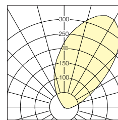
1 x 36 W lamp diffuser PMMA, clear, impact strengthened, asymmetric beam
